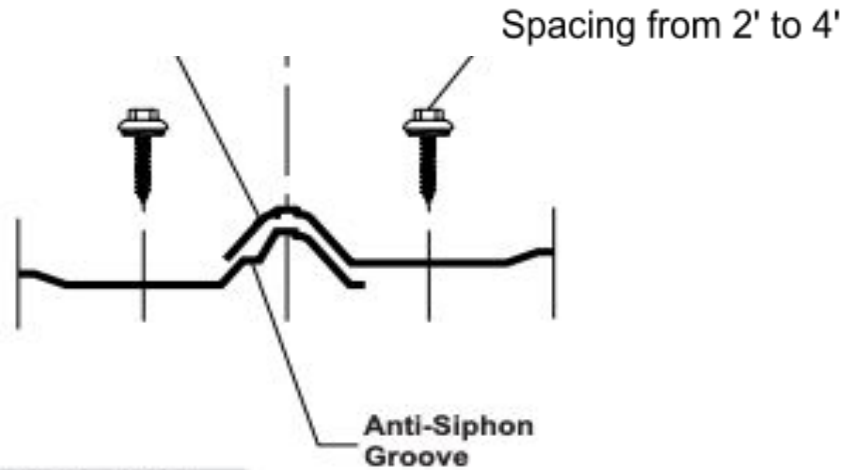
FASTENING PATTERN
